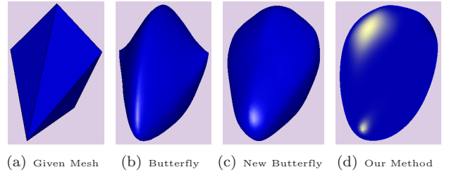
Figure 1: Comparison with Butterfly and modified Butterfly methods.
