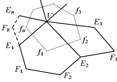
Figure 6: Vertex \mathbf{V} and its neighboring vertices.
