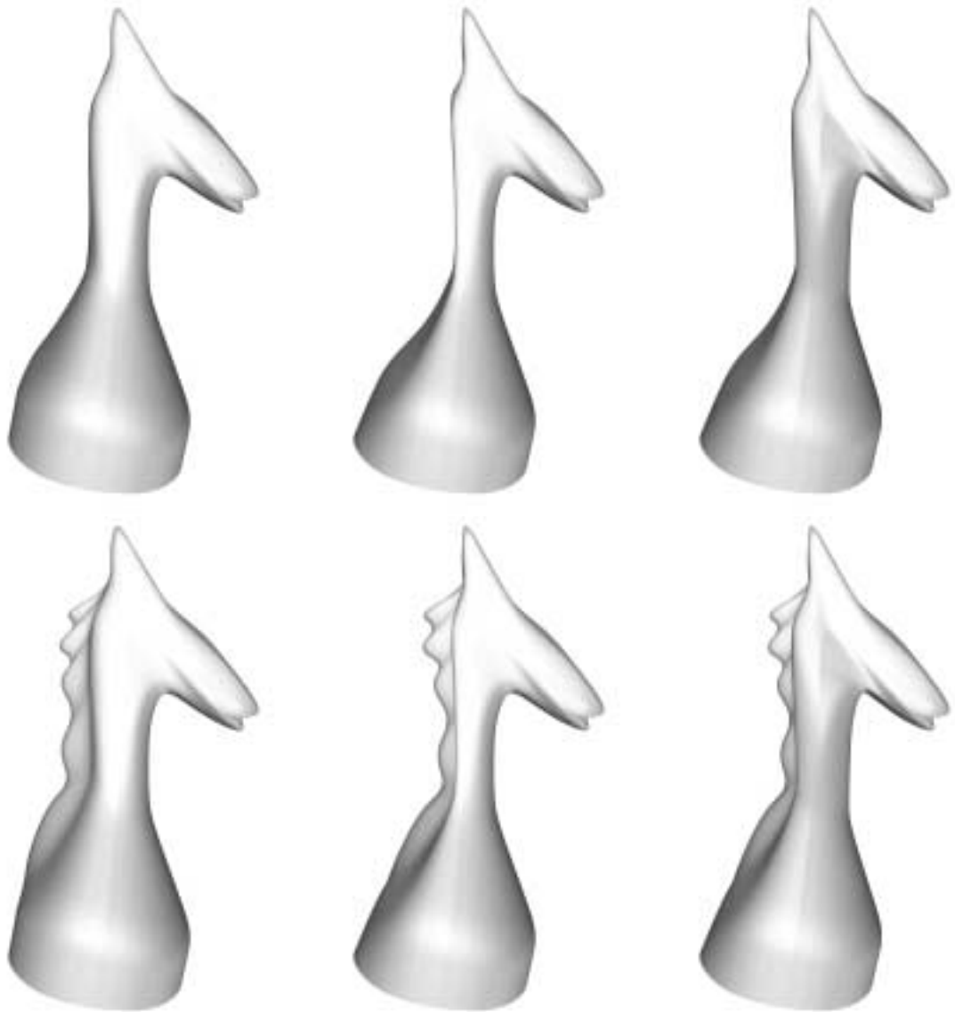
Figure 6: Deformation of a uniform B-spline surface. Left: Initial surfaces. Middle: The volume is free. Right: The volume is preserved.
