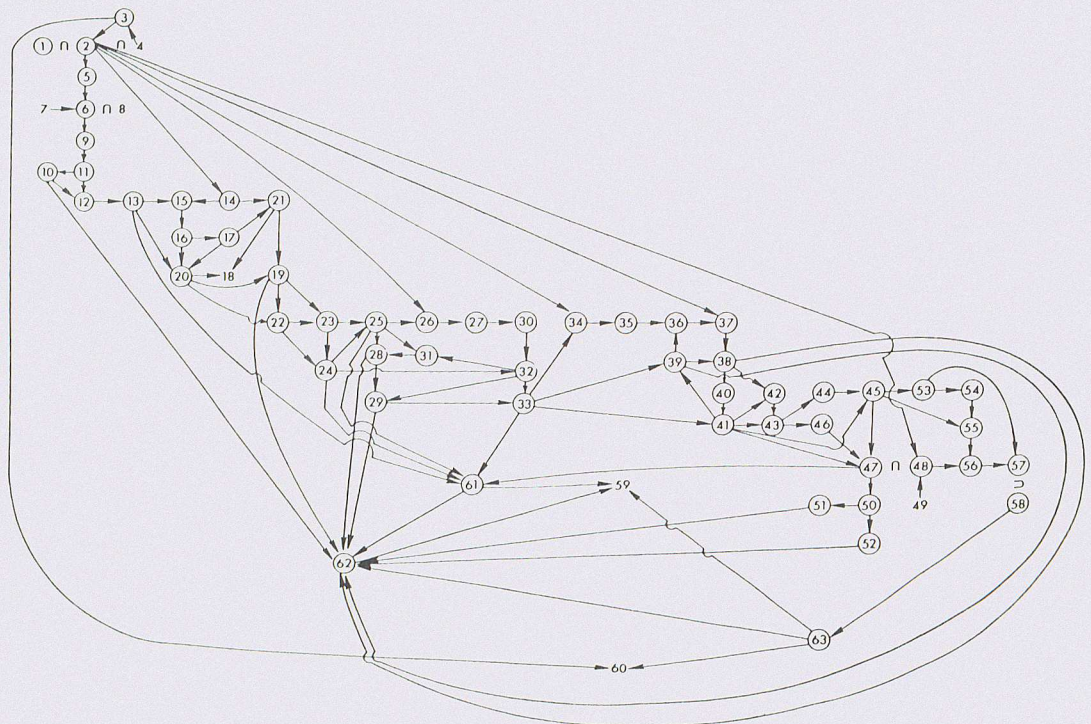
FIG. 1. Causal network representation for The Father, His Son and Their Donkey story.
