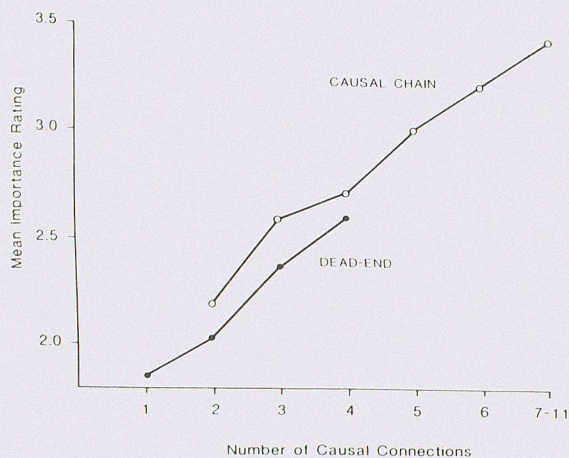
FIG. 2. Average importance judgment values for dead-end and causal chain statements that vary in the number of direct causal connections.
